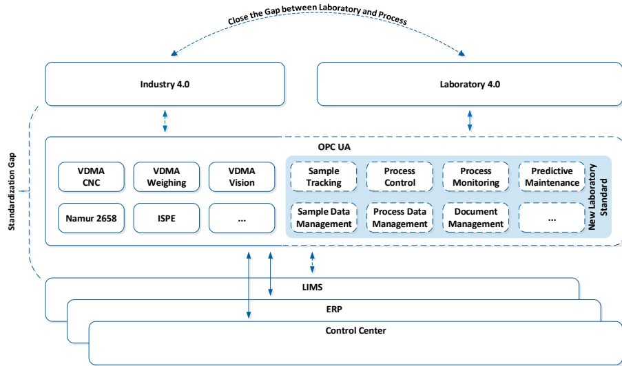
Figure 2: Integration of LADS activities in the OPC UA environment
