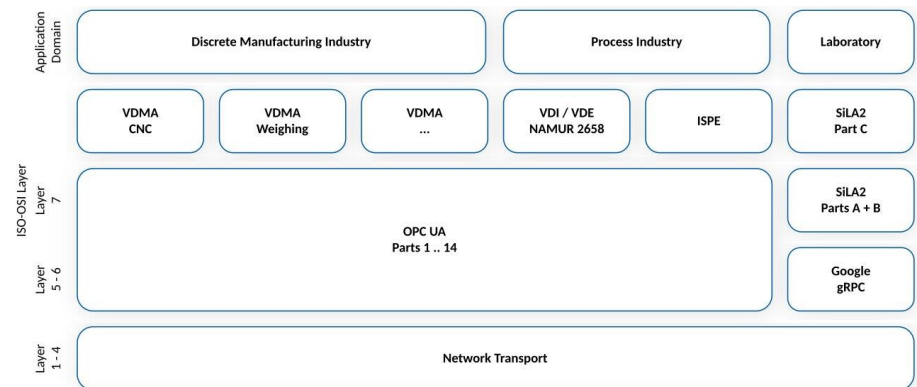
Figure 1: Assignment of existing standardisation environment into the ISO-OSI layer model
