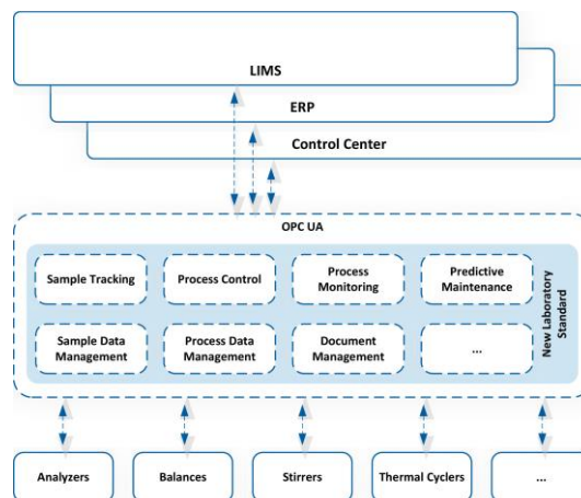
Figure 3: Approach to solving the problem of a standard, model-independent information model
